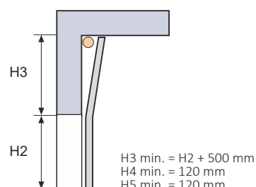
VERTICAL IND-VL
